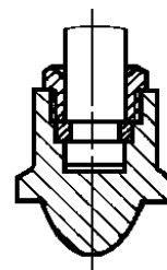
Drosselkegel throttling plug
